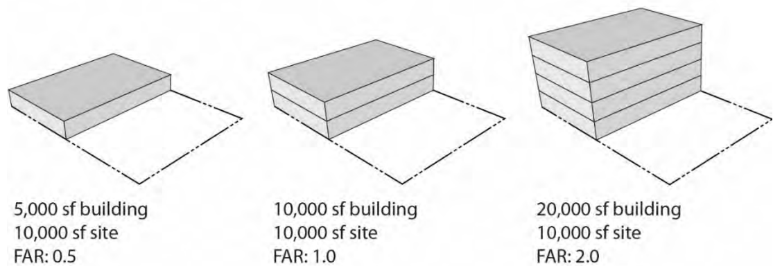
Figure LU-1: Calculating Floor Area Ratio
