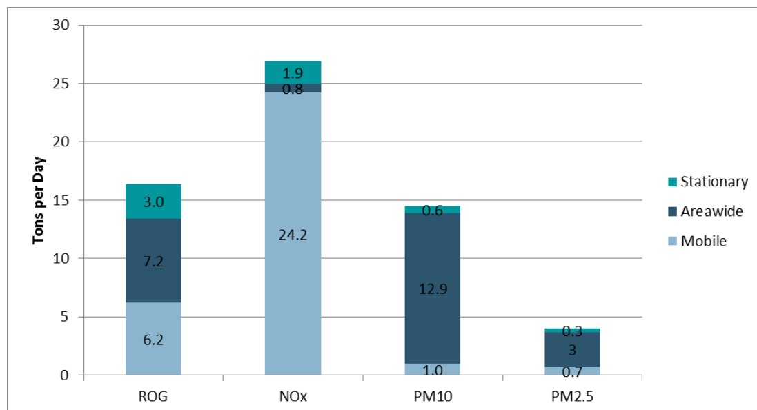
Figure C-4: San Luis Obispo County 2015 Emissions Inventory – Criteria Air Pollutants
